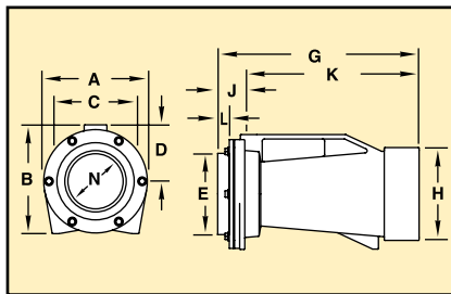
Model 905 dimensions
