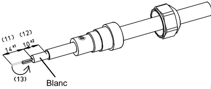
Illustration 3: finition du câble coaxial
