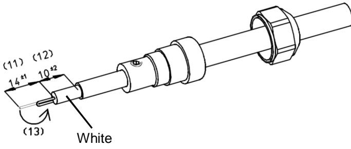
Figure 3: Coax cable finish
