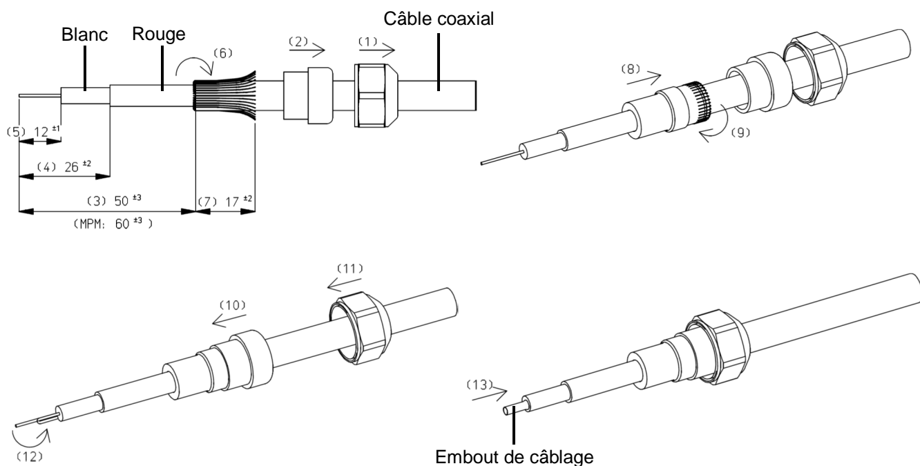
Illustration 2: finition du câble coaxial
